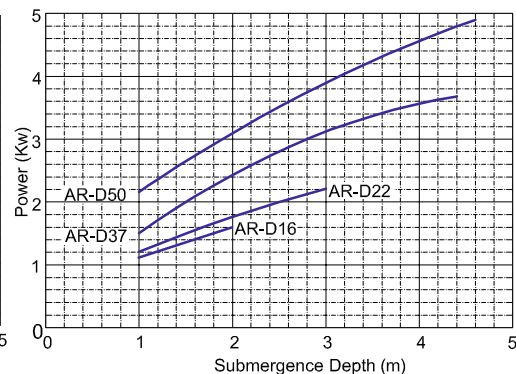
Power Curve
