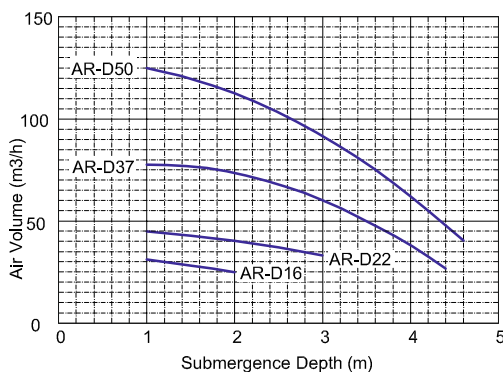
Air Volume Curve
